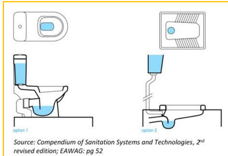
Figure 9: Cistern Flush Toilet
